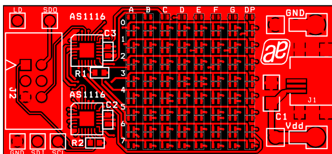
Figure 4: Top Layer
