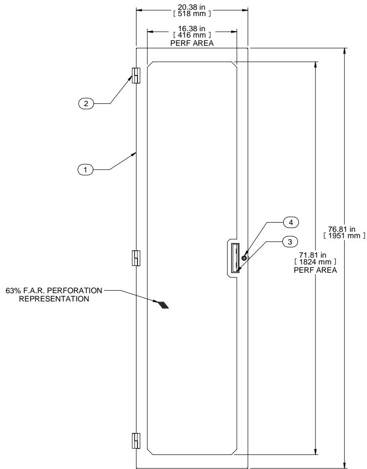
FRONT VIEW
